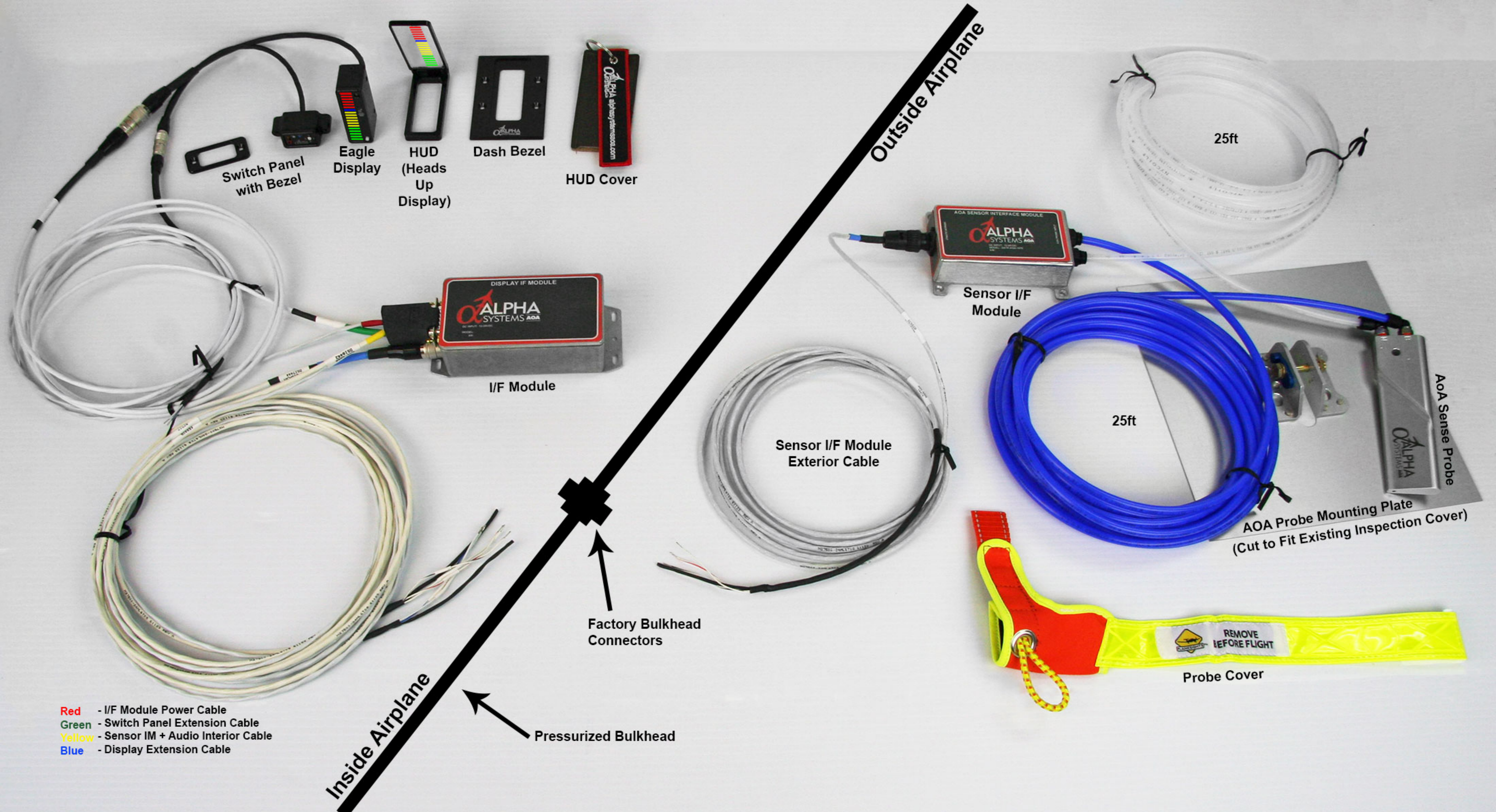
Alpha Systems AOA Falcon HUD Pressurized System Diagram DSTR-AOA-9200PK-(HUD)
